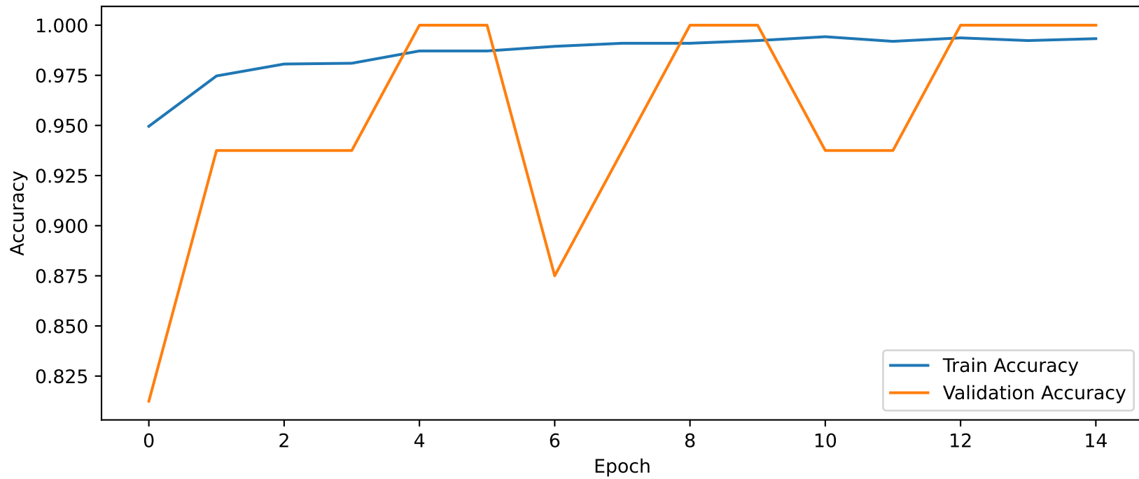
Training vs Validation Accuracy Full Fine-Tuning
